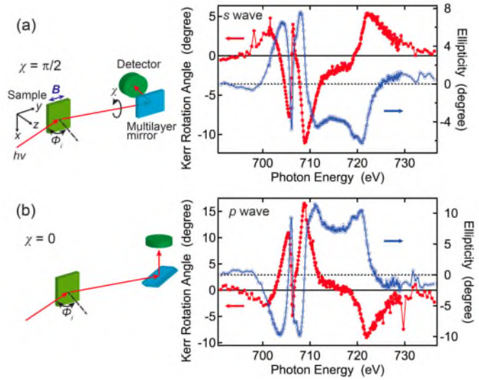
FIG. 1. Experimental setups and results of L-MOKE measurements with the polarization-modulated light for (a) the s wave and (b) the p wave. Taken from [6].
