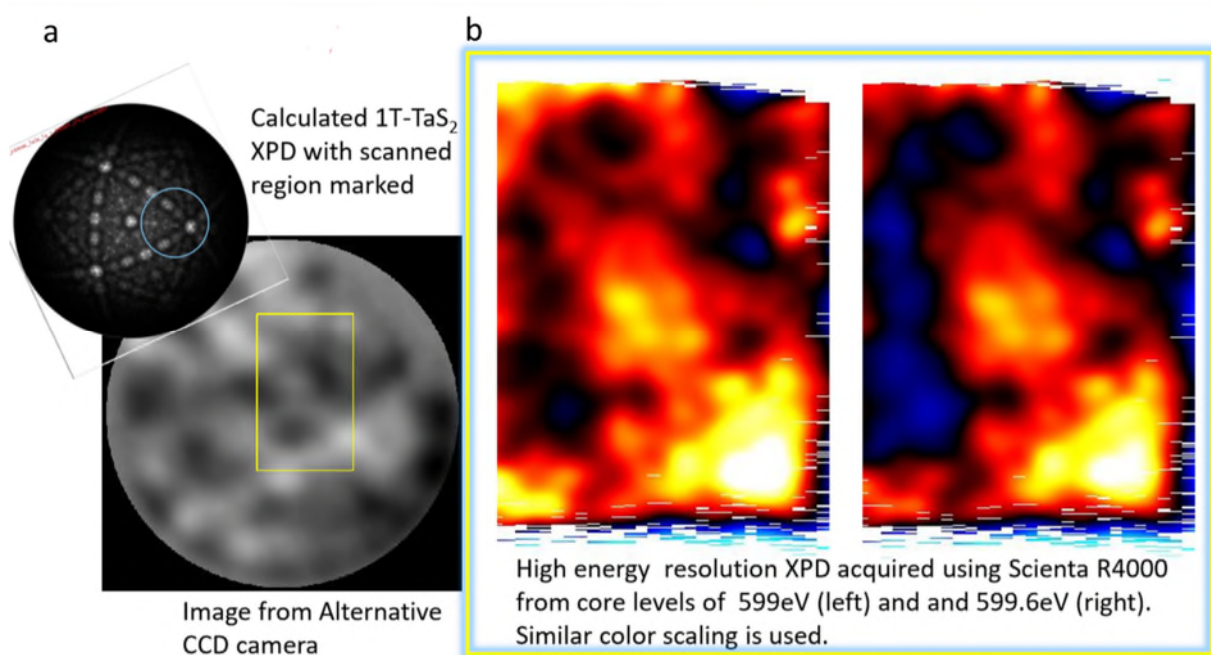
Fig. 1 (a) The experimental data obtained using DELMA without high resolution energy filtering, which is compared to the calculated 1T-TaS 2 (inset). It is noteworthy that the image was obtained within 15 seconds with good signal-to-noise ratio. (b) The stitched slices of the high energy resolution data obtained on the CCD of R4000 using the electron deflector of DELMA in front of the entrance slit of R4000. The region swept was highlighted by a rectangular box in (a).
