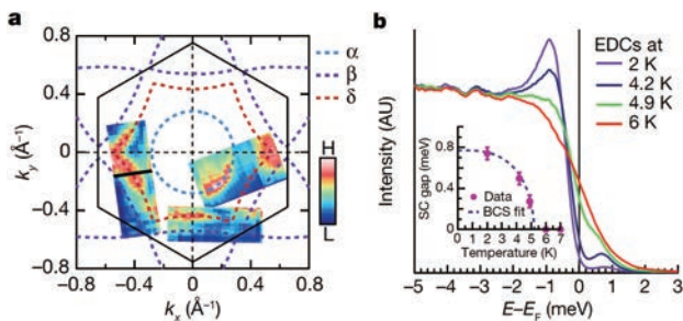
カゴメ超伝導体 \text{Cs}(\text{Va},\text{Ta})_3\text{Sb}_5 ( T_c = 5.2 \text{ K} ) のフェルミ面と超伝導ギャップ Fermi-surface map and superconducting gap of the Kagome superconductor \text{Cs}(\text{Va},\text{Ta})_3\text{Sb}_5 ( T_c = 5.2 \text{ K} )
