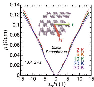
Magnetoresistance of a single crystal of black phosphorus under multiple extreme conditions. Inset shows schematic illustration of the crystal structure. Resistance along the c axis was measured in magnetic fields applied along the a axis. We observed huge positive magnetoresistance larger than 1,000 times of the value at zero field together with superposed Shubnikov-de Haas oscillations.
