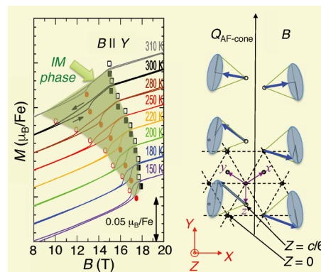
(left) Magnetization curves of single crystals of BiFeO 3 . Anomalies of magnetization curves shown in the shaded area suggest emergence of a novel multiferroics phase (IM phase) in this field-temperature region. (right) Schematic illustration of the spin arrangement in the IM phase.
